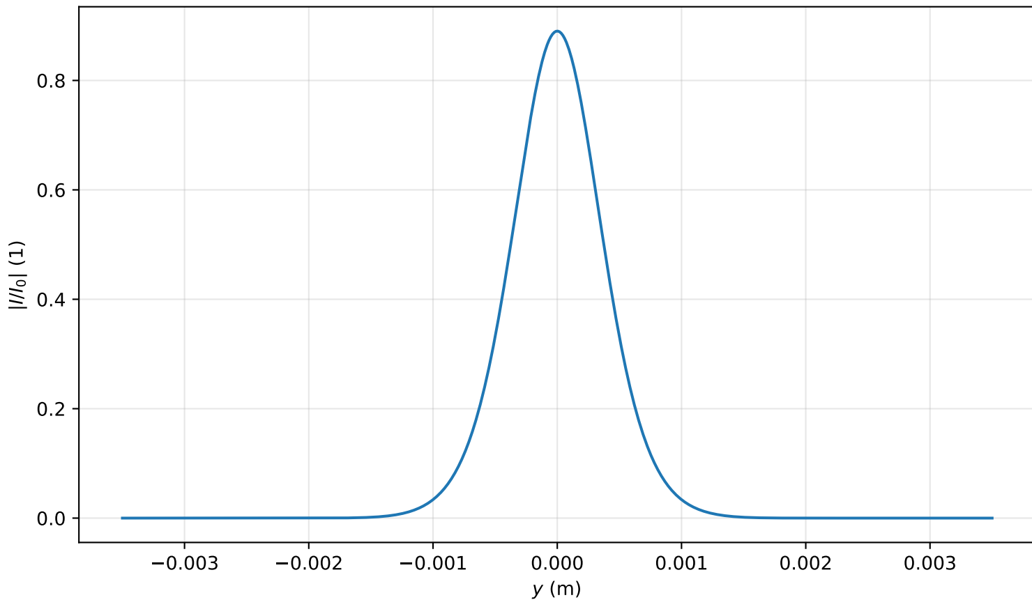
Intensity profile I(x=0, y, z=1.433)/I_0 , P_{in}=0.4P_{cr} , artificial time
